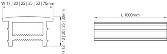
section view
