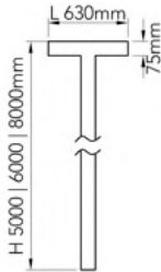
front view *height can be customized upon request
