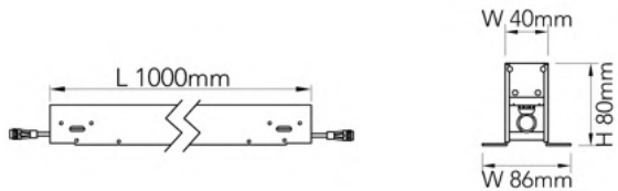
side view *length can be customized upon request
