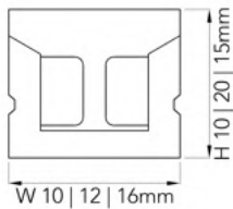
section view
