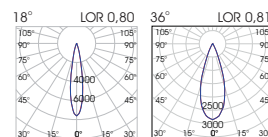
SIENA S-S7-07- 30C-90-18-BL-230ND
