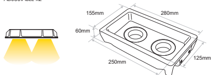
PCR.006 SEAMLESS SQUARE ADJUSTABLE x2
