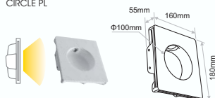
PWR.004 CIRCLE PL
