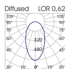
SIENA S-AC-07- 30C-90-DF-BL-230ND
