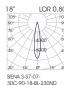
SIENA S-S7-07- 30C-90-18-BL-230ND
