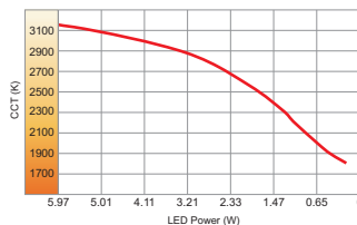
Warm dimming 3000K to 1800K (6W)
