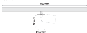
Monochromatic & TW 230VAC WL
