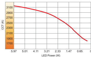
Warm dimming 3000K to 1800K (6W)
