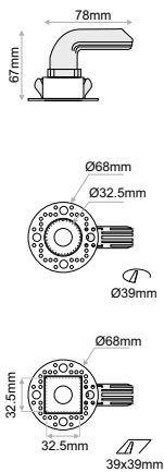
IDC.022 Trimless base for round version
