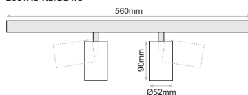
Monochromatic & TW 230VAC ND/DL/WL
