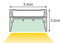
PRH.020 ANTISLIPPER for vertical installation (as extra)
