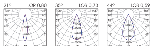
Tunable White 12W/17W
