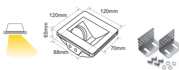
PCR.003 SEAMLESS SQUARE WASH 45°
