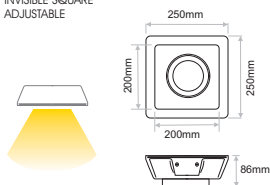
PCR.011 INVISIBLE SQUARE ADJUSTABLE
