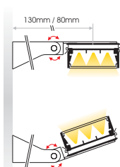
WALL BRACKET (Long/Short)
