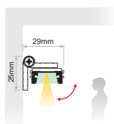
SURFACE B Installation
