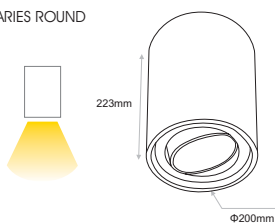
PCS.004 ARIES ROUND
