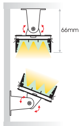
SURFACE
