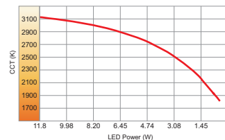
Warm dimming 3000K to 1800K (12W)
