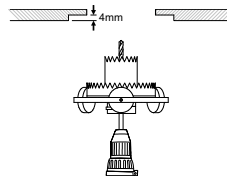
ACR.313 Tool for REFORM 52 IN-OUT TR without case
