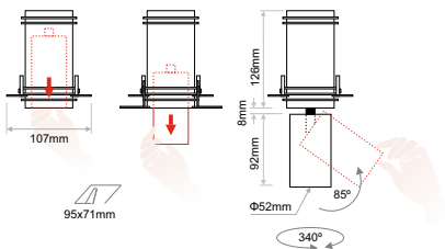
ACR.313 Tool for REFORM 52 IN-OUT TR without case
