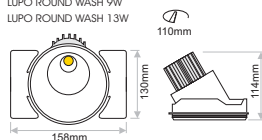
LUPO ROUND WASH 9W LUPO ROUND WASH 13W
