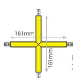
LINILINE SP PDDI-XT X Type extension.
