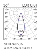
SIENA S-S7-07- 30B-90-36-BL-230ND
