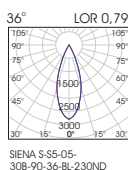
SIENA S-S5-05- 30B-90-36-BL-230ND
