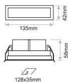
LIMA Diffused Recessed 10
