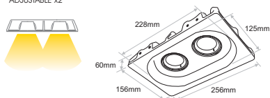
PCR.009 SEAMLESS ROUND ADJUSTABLE x2
